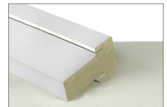
MULL POST W/O LVL 1-1/2" X 3-9/16" X 2-1/2" 1" X 3-9/16" X 2" 1-1/2" X 4-3/8" X 2-1/2" 1" X 4-3/8" X 2"
